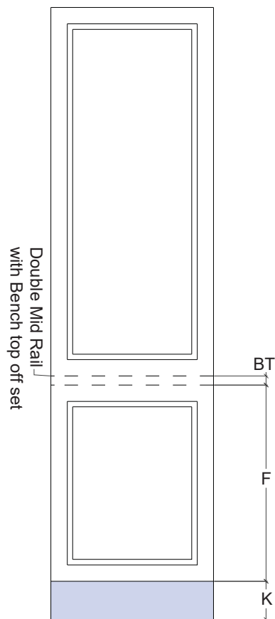
T4 - Tall Panel Type 4 Base Door Height with benchtop Thickness
