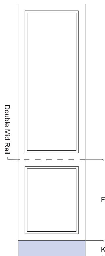
T3 - Tall Panel Type 3 Base Door Height with double Mid Rail
