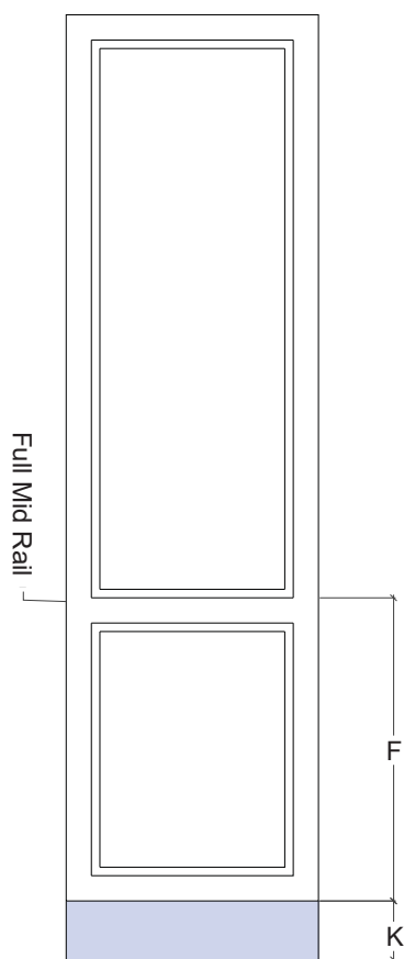
T2 - Tall Panel Type 2 Base Door Height with standard Mid Rail
